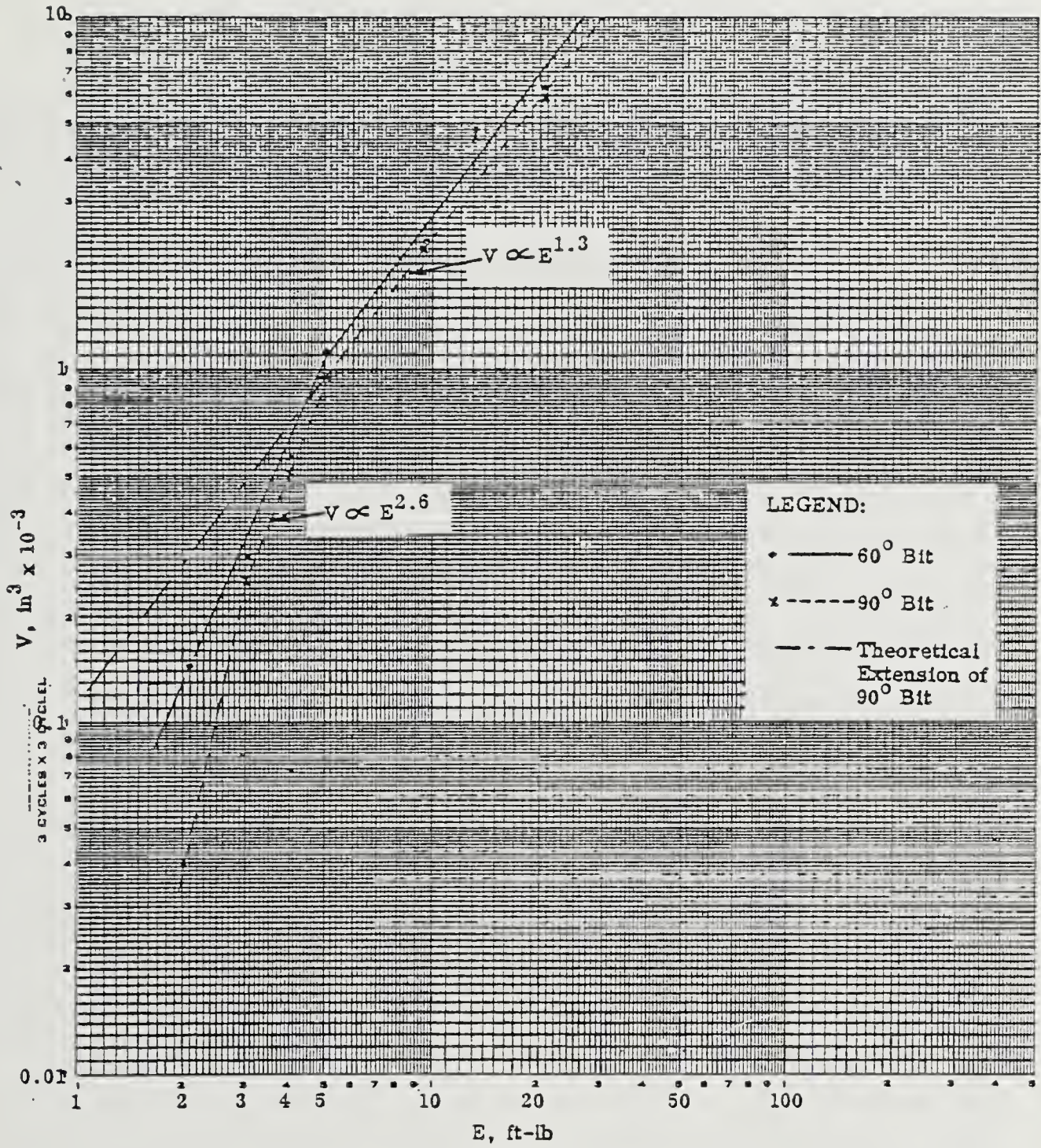
Volume-Energy Relation for 60° and 90° Wedge Bits in Drop Tests on NASA Standard Basalt Sample.
